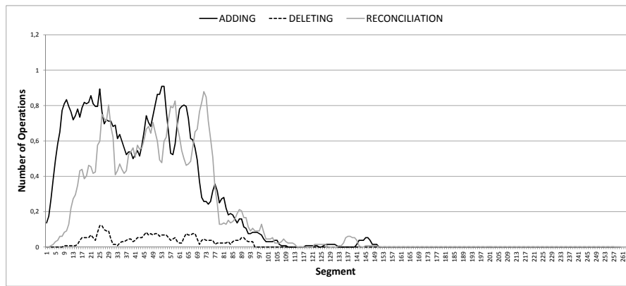
Fig. 2. Cluster C2
