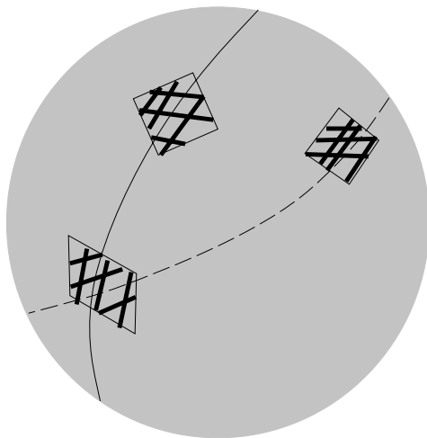
Figure 6: The geometric setting of the three viewing directions. The unknown viewing directions lie on great circles which pass through the viewing direction of the first image. The epipolar lines of each pair of images are parallel to the great circle which runs between them.
