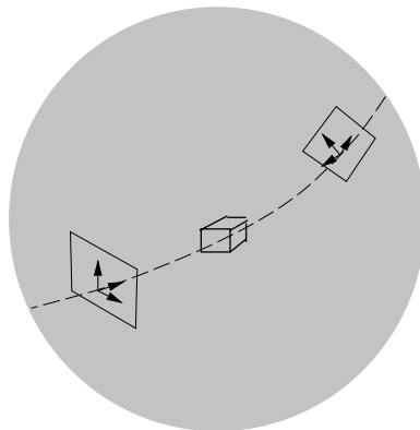
Figure 3: Recovering the viewing direction component of motion. All that can be recovered is the great circle on the viewing sphere on which the viewing direction of the second image lies.
