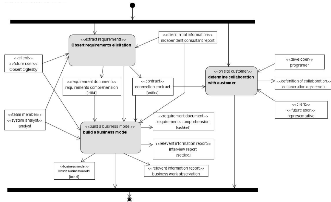
Figure 4. Part of the situational methodology which was created for Obsert's case
