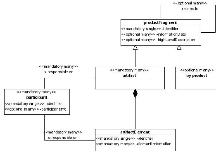
Figure 3. A description of an artifact, which is a specialization of a product fragment
