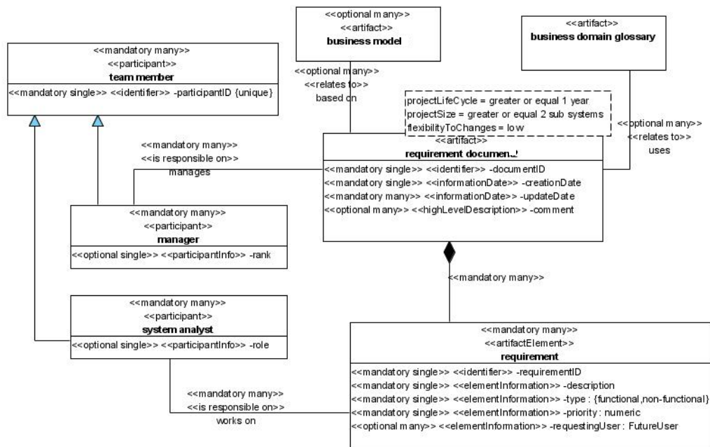
Figure 2. A description of the "requirement document" product fragment of RUP in ADOM
