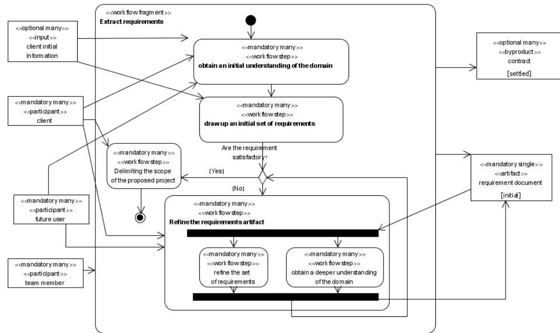
Figure 1. A description of the "extract requirements" process fragment of RUP in ADOM
