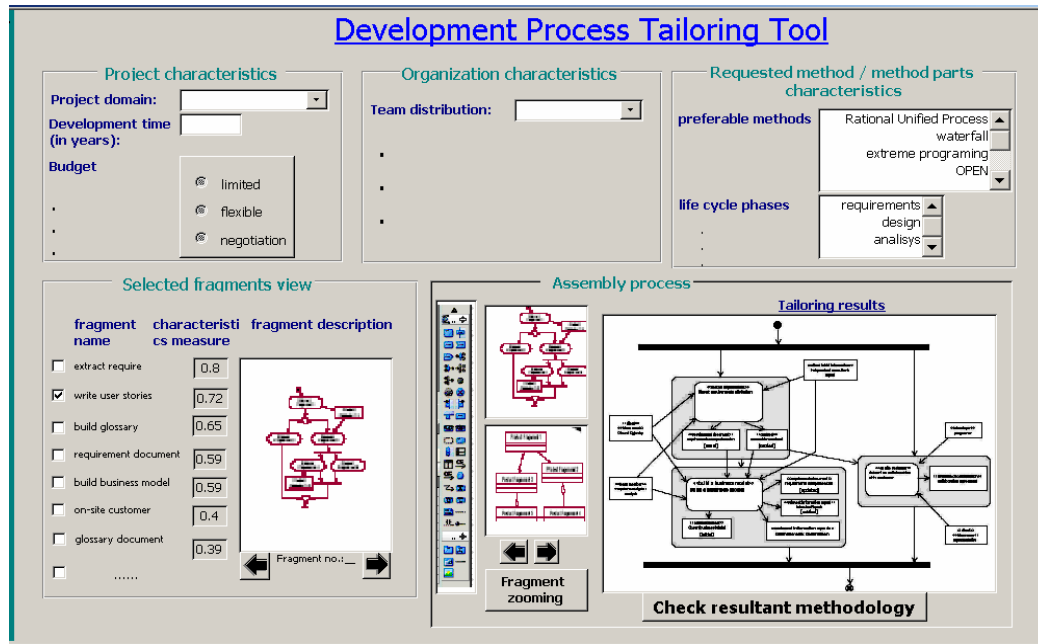
Figure 5. The supporting CASE tool interface
