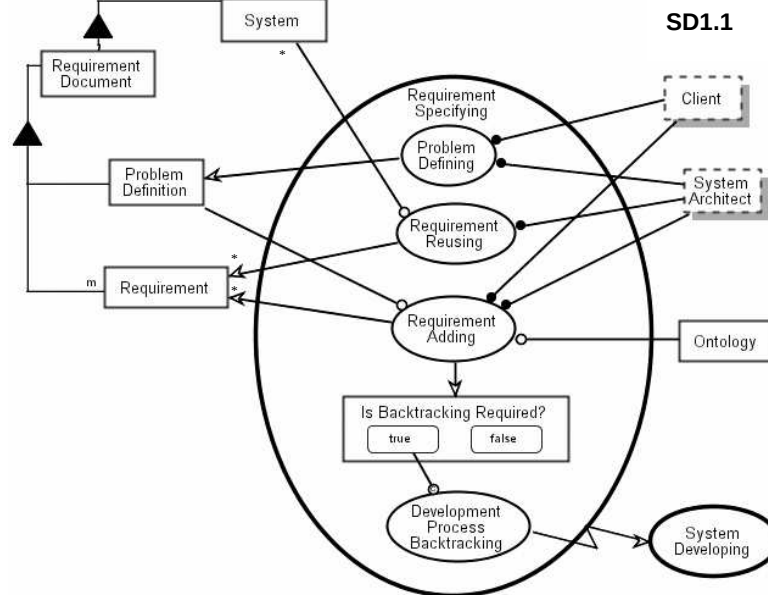
Figure 3. Zooming into Requirement Specifying
