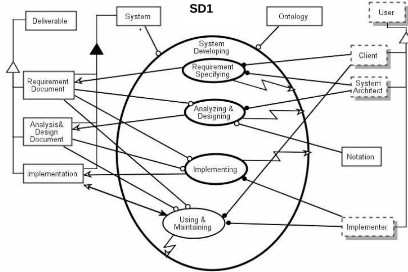
Figure 2. Zooming into System Developing
