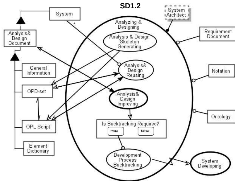
Figure 4. Zooming into Analyzing & Designing
