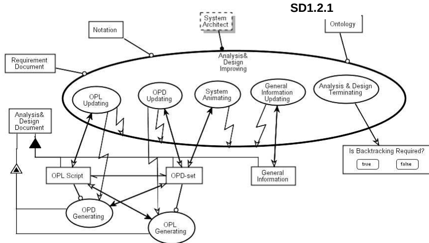
Figure 5. Zooming into Analysis & Design Improving
