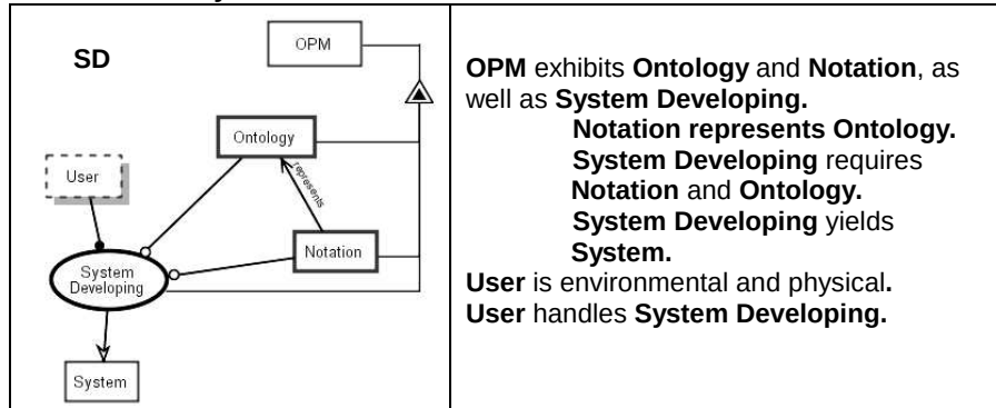
Figure 1. The top level specification of the OPM metamodel
