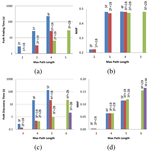
Figure 2: Path finding time (a) and MAP (b) for the KB inference (top) and name extraction (bottom) tasks. A marker iF + jB indicates the maximum path exploration depth i from query node s and j from target node t —so that the combined path length is up to i + j . No paths with constants were used.
